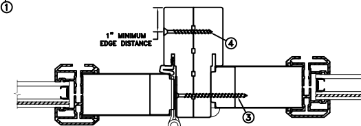
TYP. MULLION DETAIL HORIZONTAL SECTION
